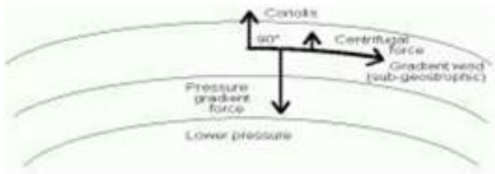
Figure 10.4: Geostrophic Wind
