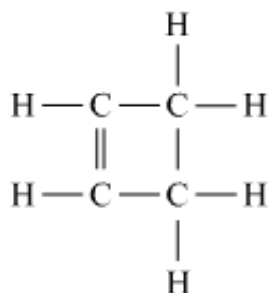
Cyclobutene
